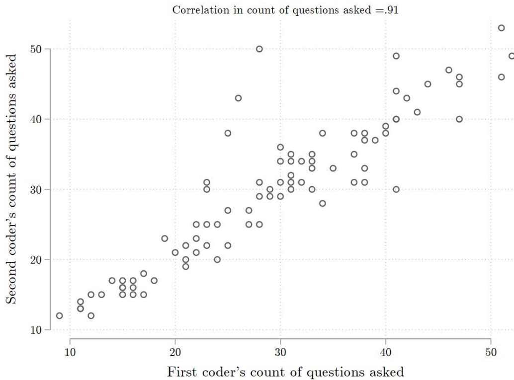
Figure 2: Inter-Coder Reliability
